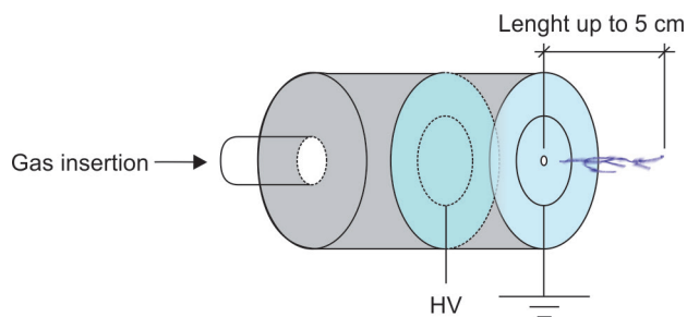
Fig. 3: A schematic of the plasma pencil created by Laroussi et al
