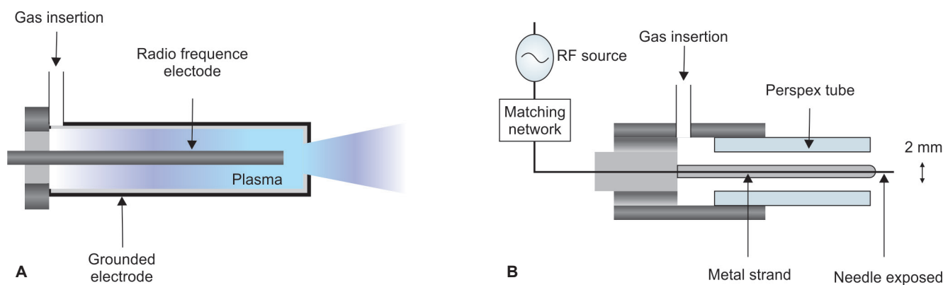
Figs 2A and B: An APPJ and a plasma needle: (A) Schematic of the APPJ created by Schütze et al in 1998; and (B) schematic of the plasma needle created by Stoffels et al in 2002
