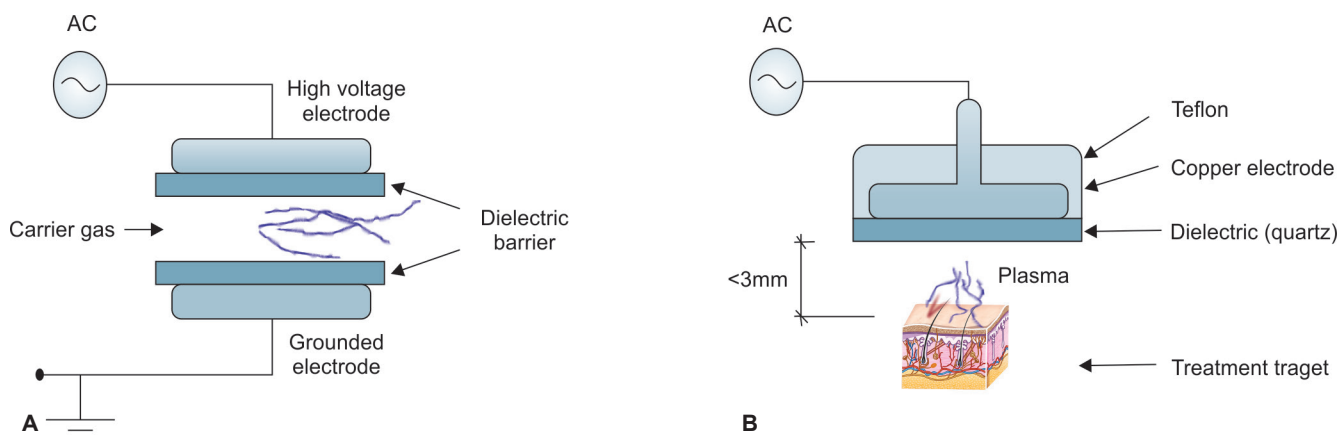
Figs 1A and B: Dielectric barrier discharge and a floating electrode dielectric barrier discharge (FE-DBD). (A) Formation of plasma by DBD; and (B) FE-DBD
